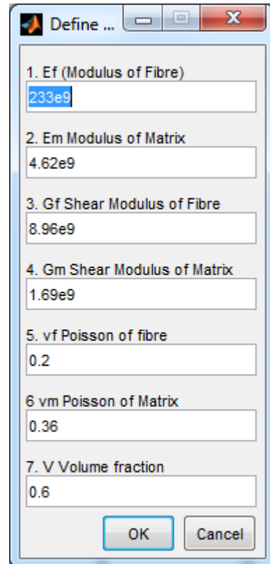
Fig. 3. Interactive interface input data
